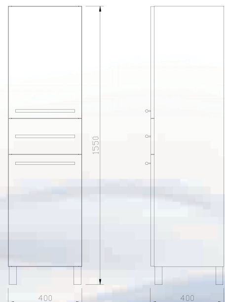
NIDA High Cabinet
