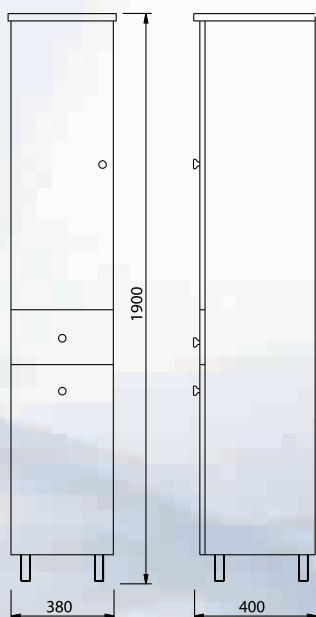
ERCE High Cabinet
