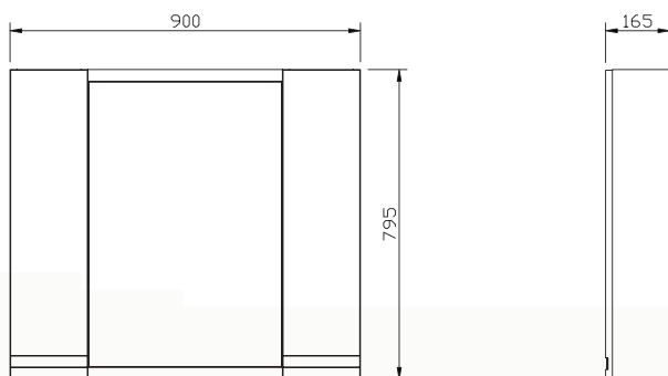
SOHO 90cm (Double Door)
