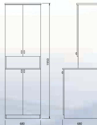
YAKUT (Single Door) Washing Machine Cabinet
