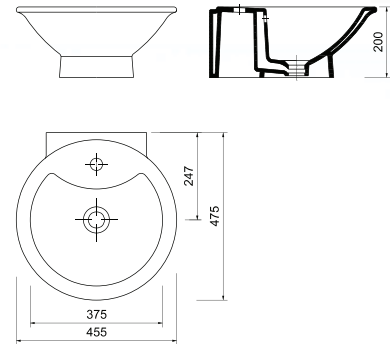
Weight: Washbasin 13 kg
