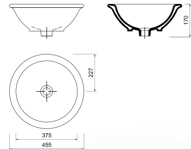
Weight: Washbasin 7,8 kg
