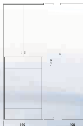
YAKUT Washing Machine Cabinet
