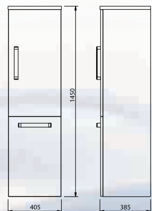
MODO High Cabinet
