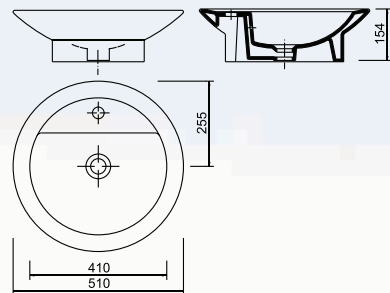
Weight: Washbasin 11,3 kg
