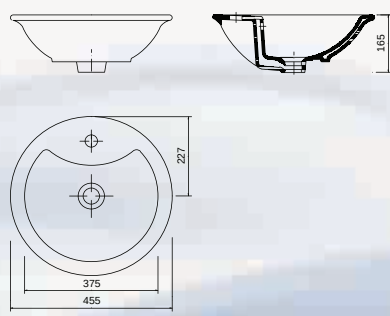
Weight: Washbasin 7,8 kg
