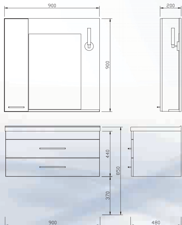
NIDA 90 Set (Single Door)
